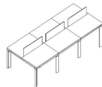
Zen sextuplo A Medidas: 360/420/480/540 x 140 x h74 cm
